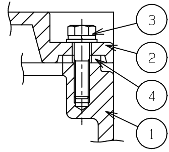
“A”部詳細図(1/3)
